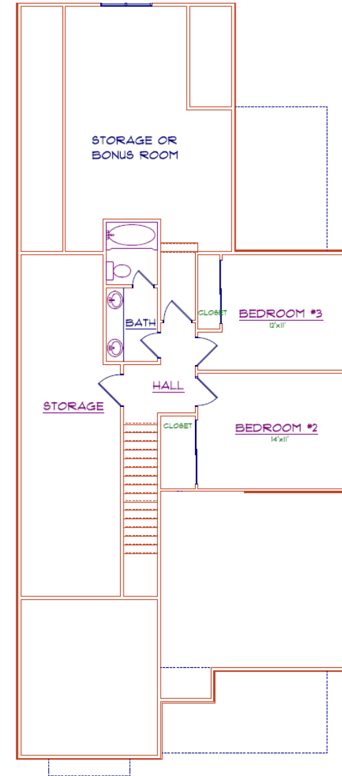
"RIVER BIRCH" 2ND FLOOR PLAN
