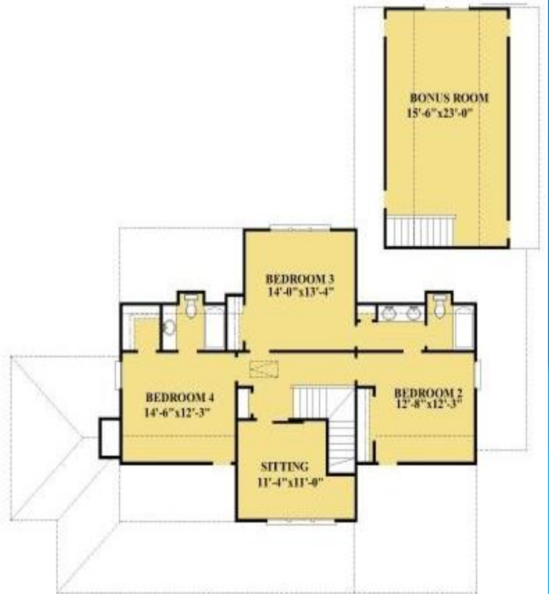
SECOND FLOOR PLAN HEATED SQUARE FEET 1510
